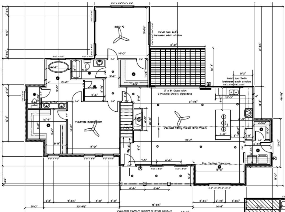
MAIN FLOOR SCALE: 1/4" = 1'-0"
